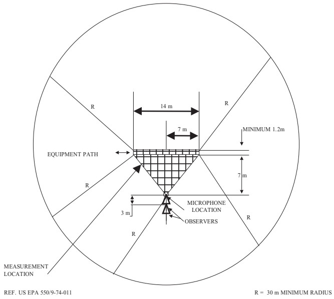
TEST SITE CONFIGURATION FOR EXTERIOR SOUND LEVEL MEASUREMENT PROCEDURE FOR SMALL ENGINE POWERED EQUIPMENT - SAE J 1046
